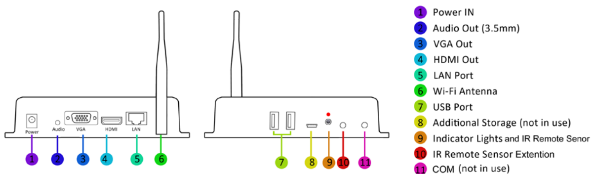
Figure 1 Product Overview
