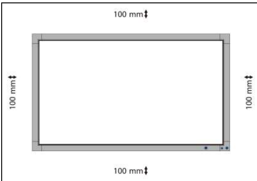
Figure 3 Ventilation Area
